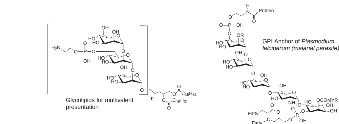
Fig. 1. Some NPOE derived oligosaccharides.
